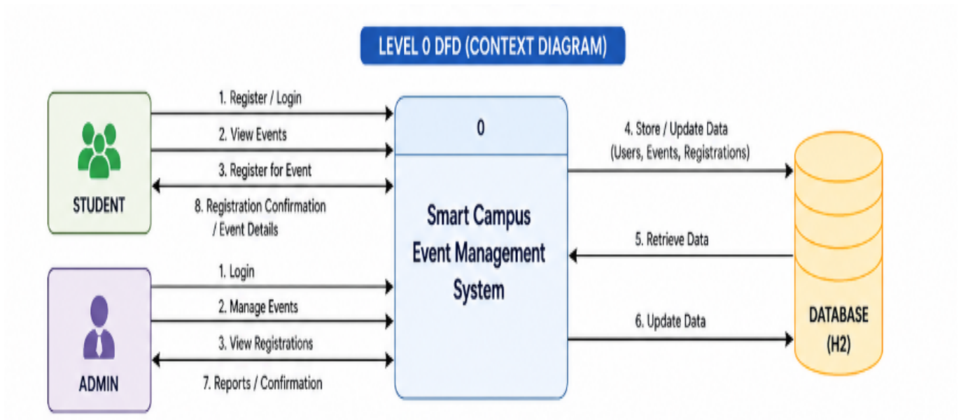
Figure 4.2: Data Flow Diagram Level 0: Context Diagram
