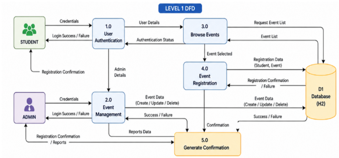
Figure 4.3: Data Flow Diagram Level 1: Functional Decomposition
