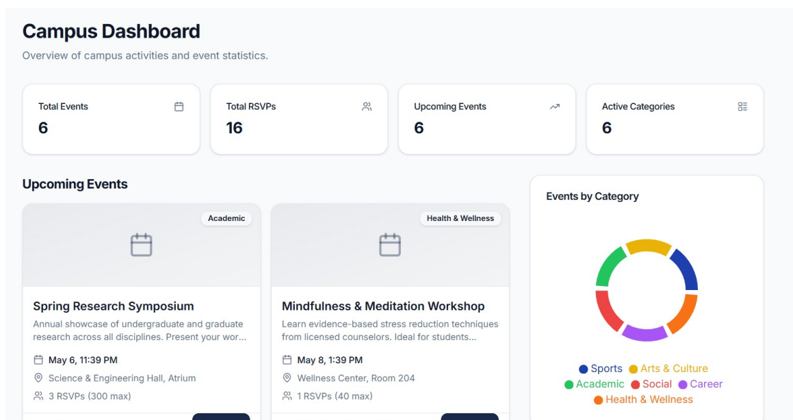
Figure 5.4: Admin Dashboard
