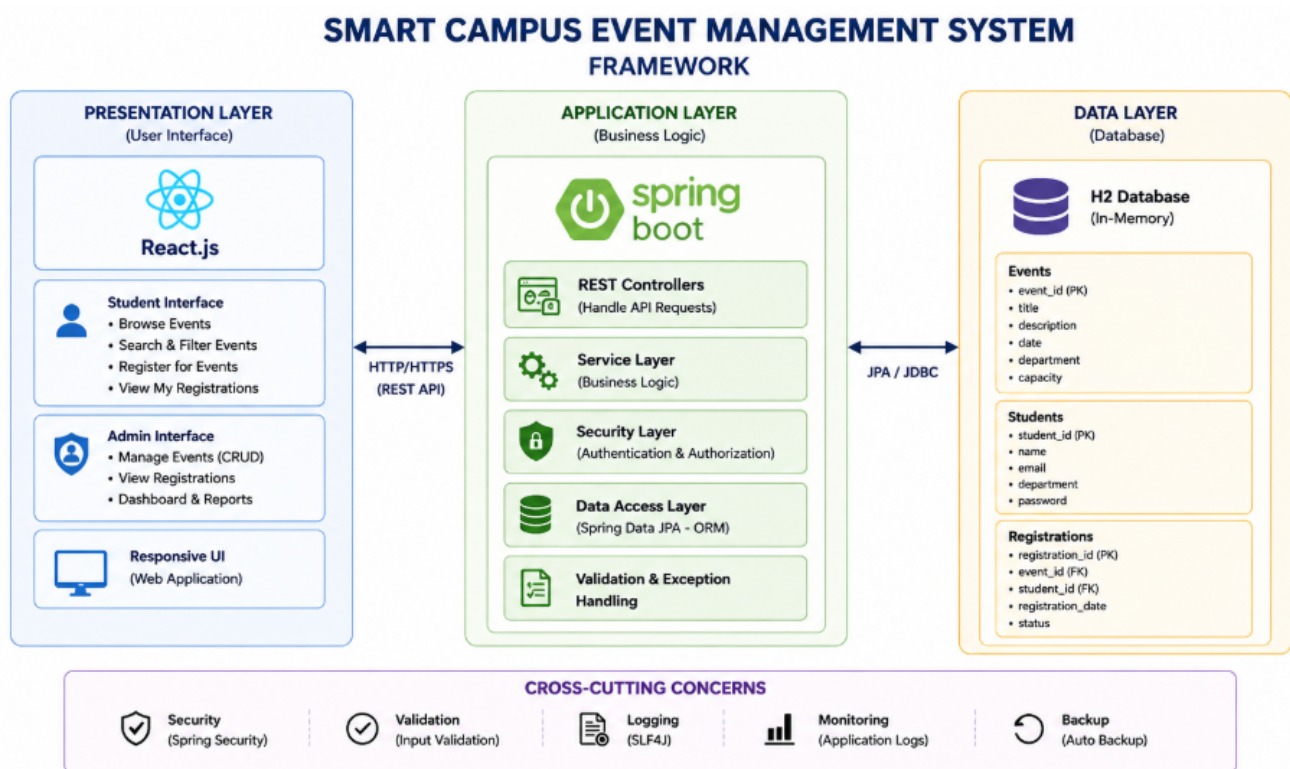
Figure 1.1: Framework
